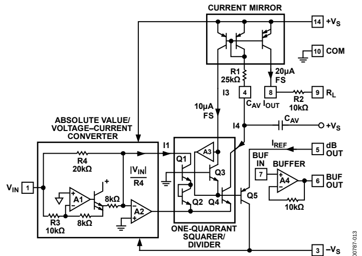
Figure 7. Simplified Schematic
